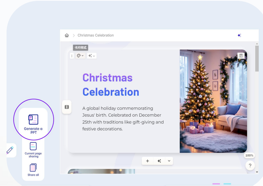
• PPT Generation
