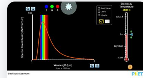
Blackbody Spectrum
