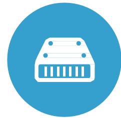
Save Storage
