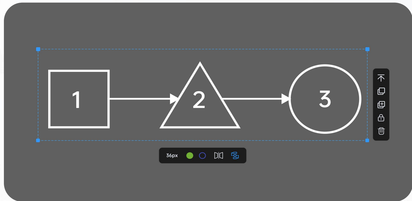
• Flowchart Generation
